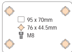
75mm swivel
