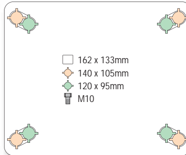
125, 150mm swivel
