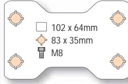
75mm fixed
