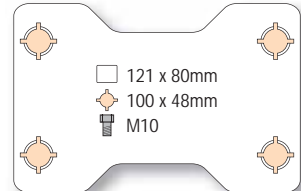
100, 125mm fixed
