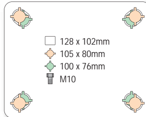
125, 150mm swivel
