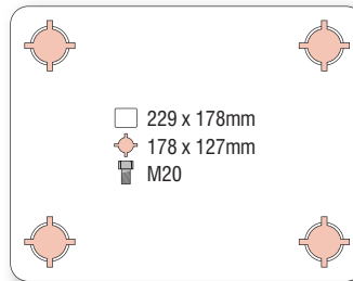
EH 516 (swivel)
