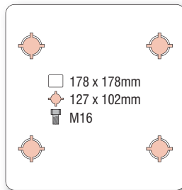
EHF 312 (fixed)
