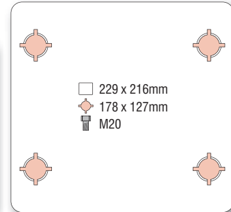
EHF 516 (fixed)
