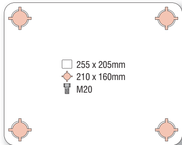
TSY (swivel)
