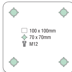
92mm swivel
