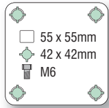
42mm swivel
