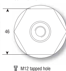
50mm swivel
