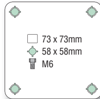
50mm swivel
