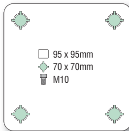
72mm swivel
